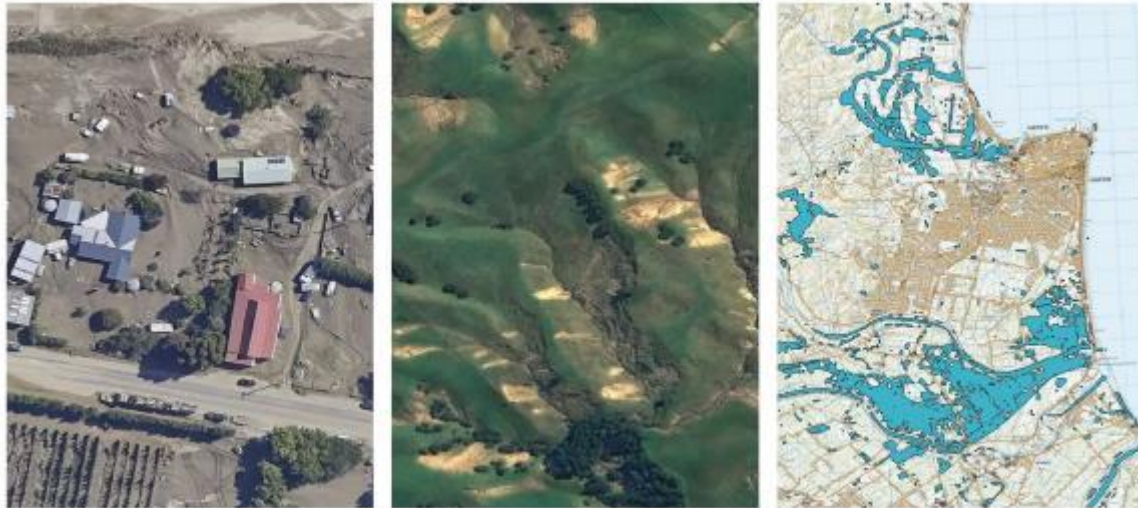
Figure 9 - Data captured during Cyclone Gabrielle including aerial imagery, satellite imagery and approximate flood extents.
