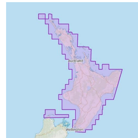
J - Cyclone Gabrielle
